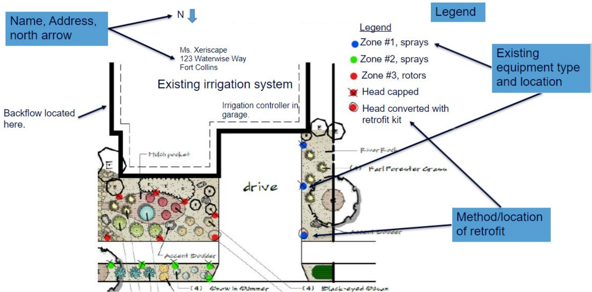
Figure 3 - Irrigation Plan Example
