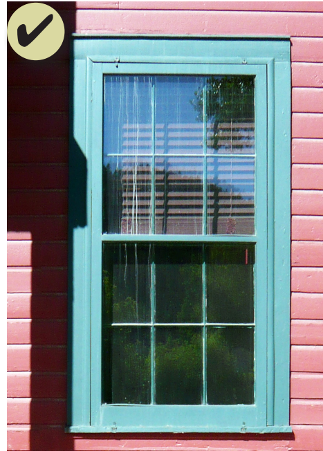
Figure 89: Use storm windows designed to match the historic window frame if placed externally.
