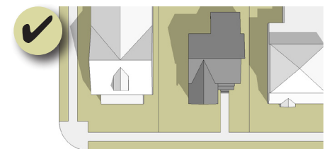
Figure 187: Locate a new building to maximize passive solar potential. This example illustrates a building (top) imposing on its neighbor's solar access.
