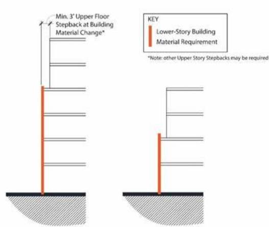
Figure 18.4 Building Base Materials
