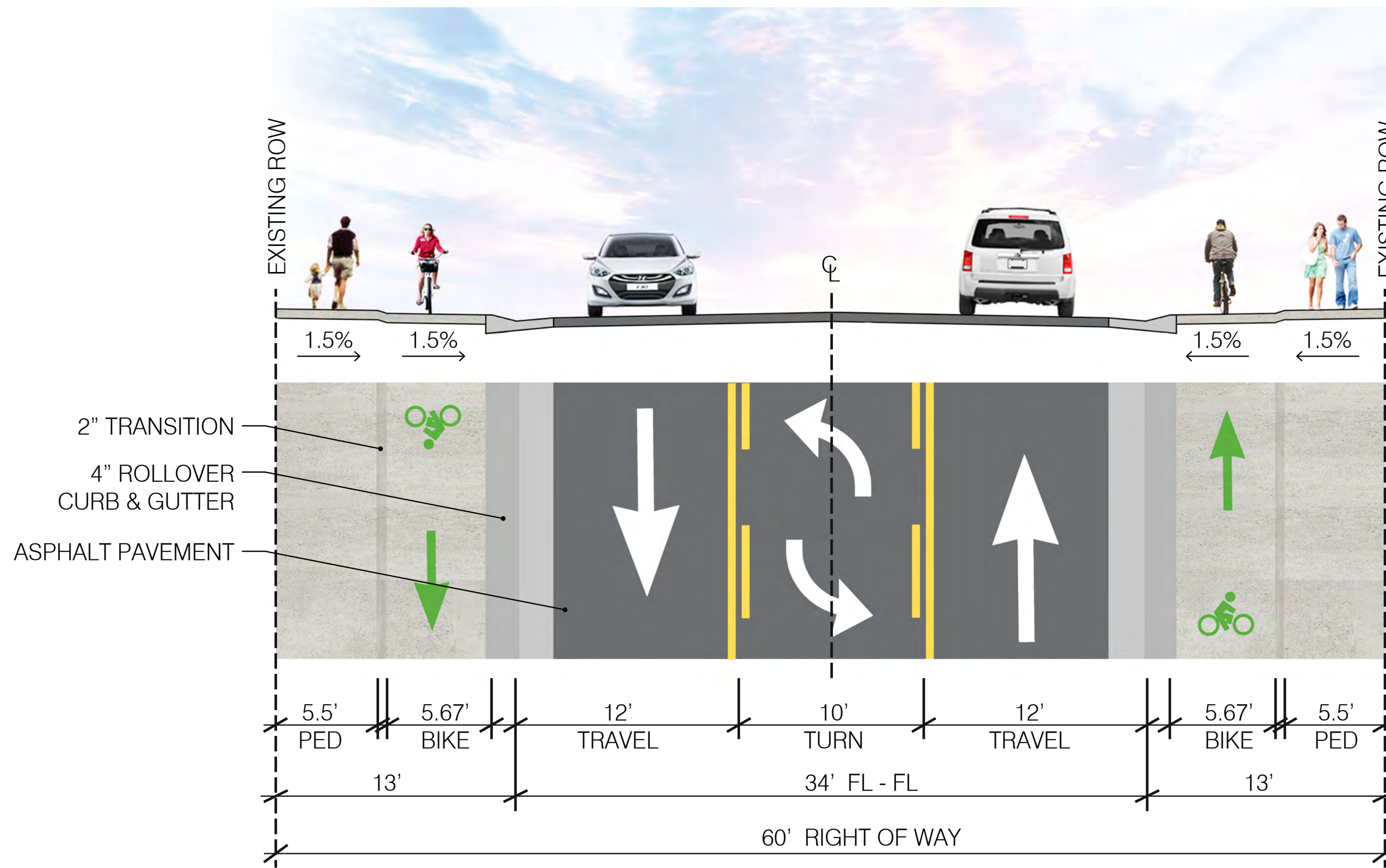
SUNSET STREET TO PSD PROPERTY STREET TYPICAL SECTION
