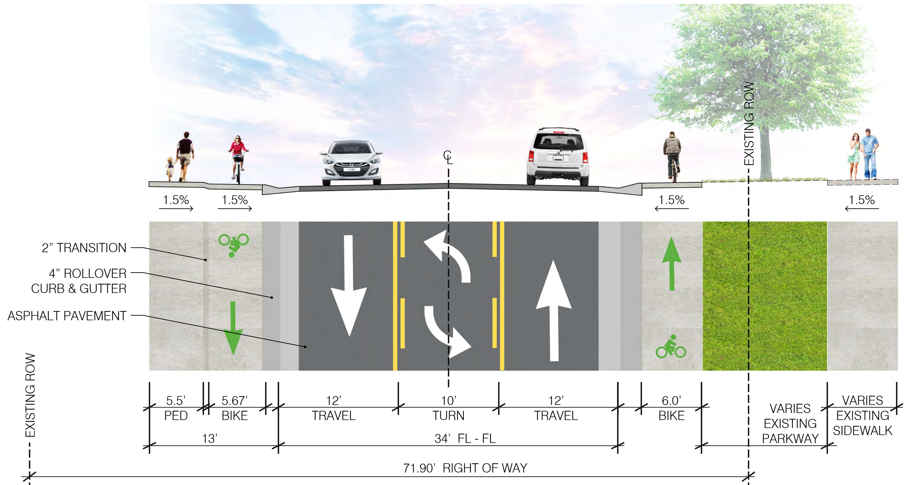
PSD PROPERTY TO TAFT INTERSECTION STREET TYPICAL SECTION
