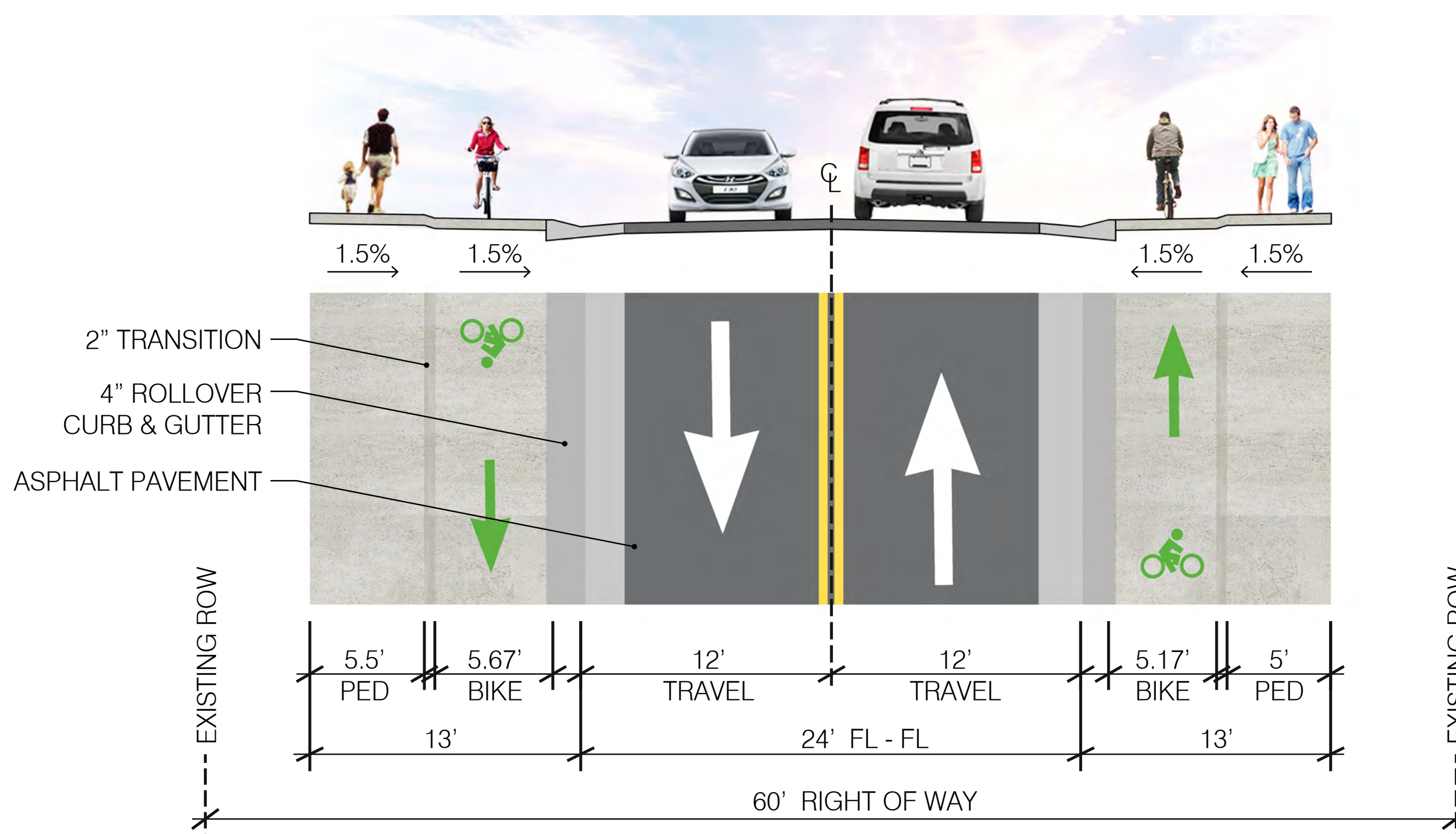
TAFT INTERSECTION TO EASTERN NEW MERCER CANAL CROSSING STREET TYPICAL SECTION
