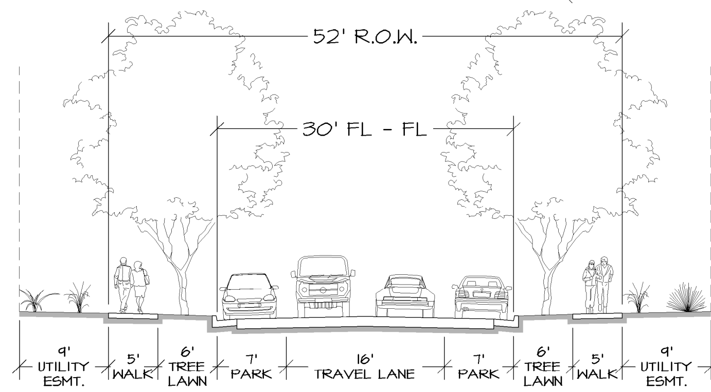
A GREEN LAKE DRIVE (RESIDENTIAL LOCAL STREET) SCALE: 1" = 10'
