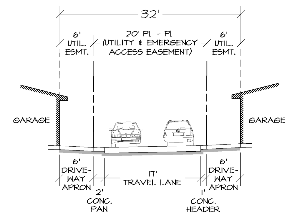
B PRIVATE DRIVE SCALE: 1" = 10'
