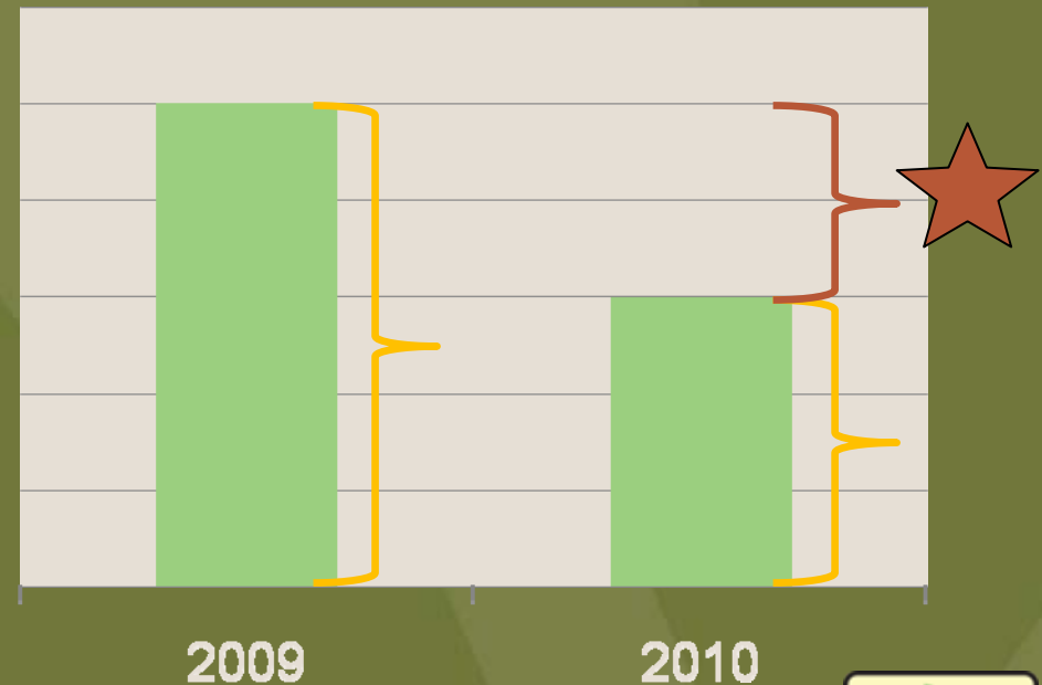
Annual GHG Emissions
